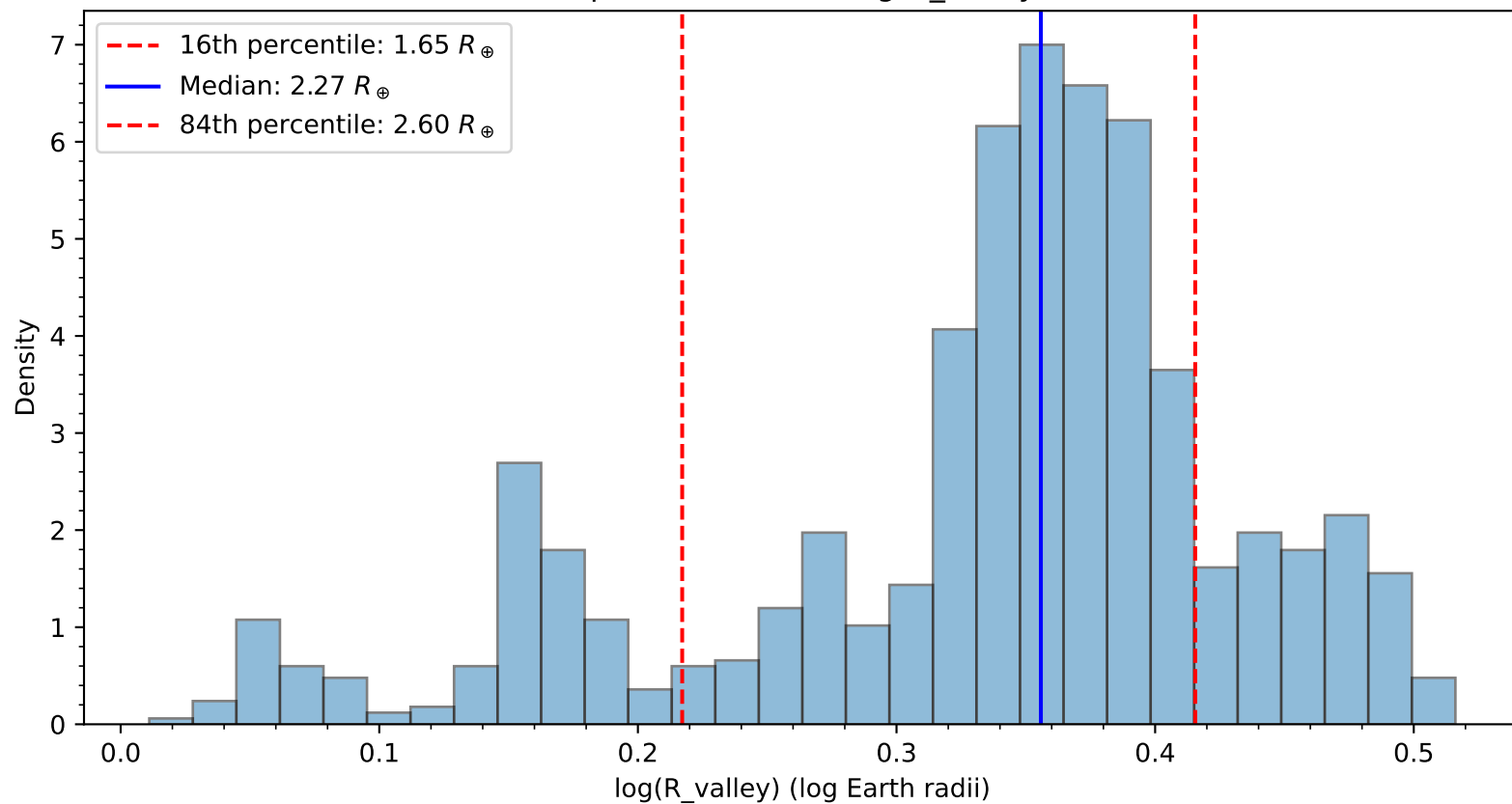
Bootstrap Distribution of \log(R_{\text{valley}}) , bin 1
